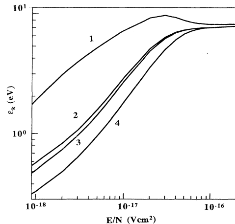
FIG. 3. Characteristic energy \varepsilon_k vs E/N for conditions of Fig. 1. \varepsilon_k = D/\mu , D is the electron transverse diffusion coefficient, \mu is the electron mobility.
